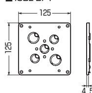
■4CBL-BPY
