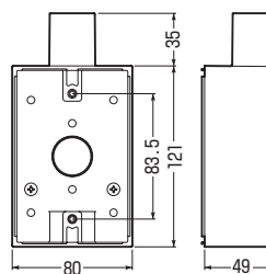
■PVR22-BC2□
