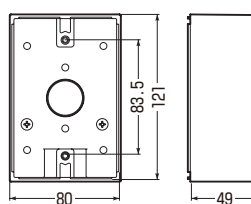
■PVR22-BC1A□
