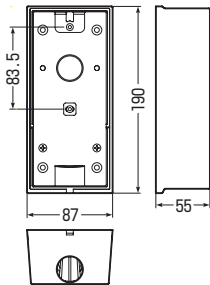
■PVR22-LBC1J
