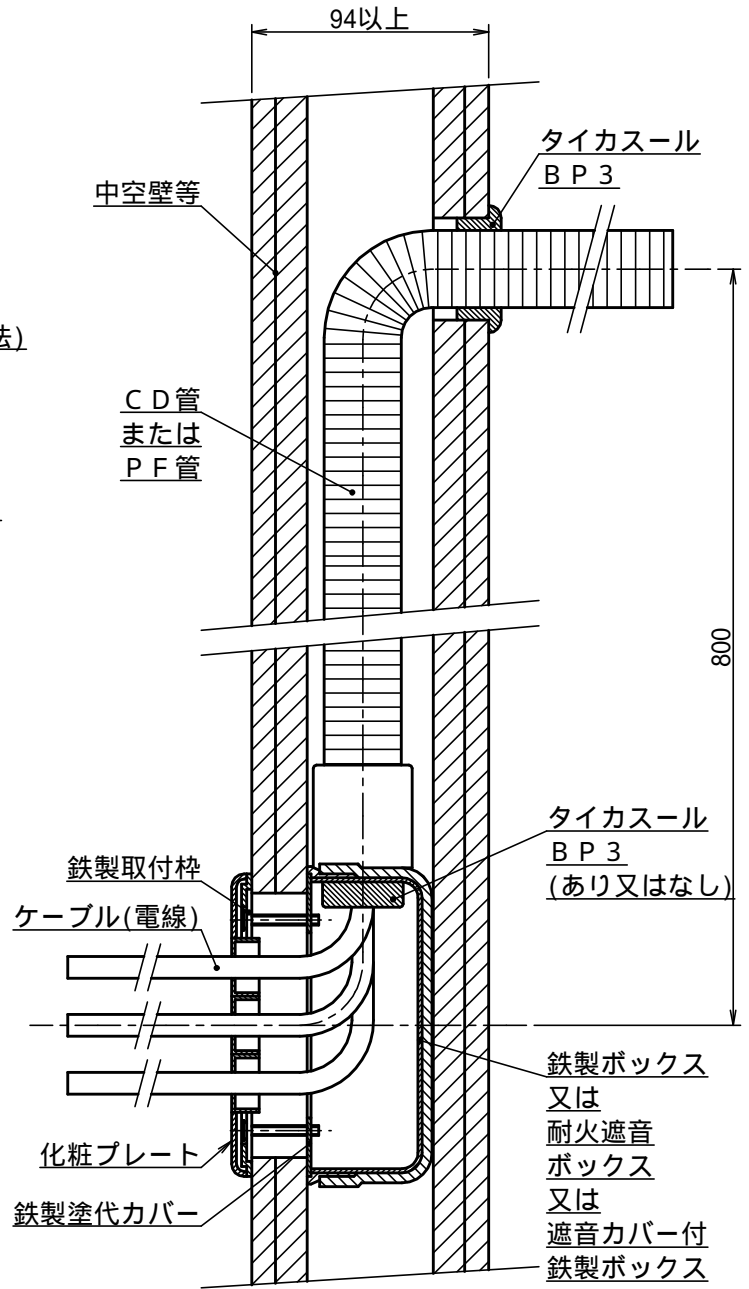
断面図(1/3)
