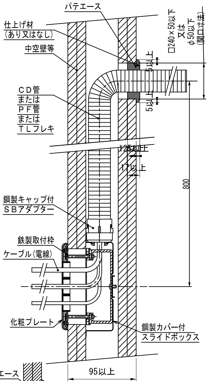
断面図(1/3)
