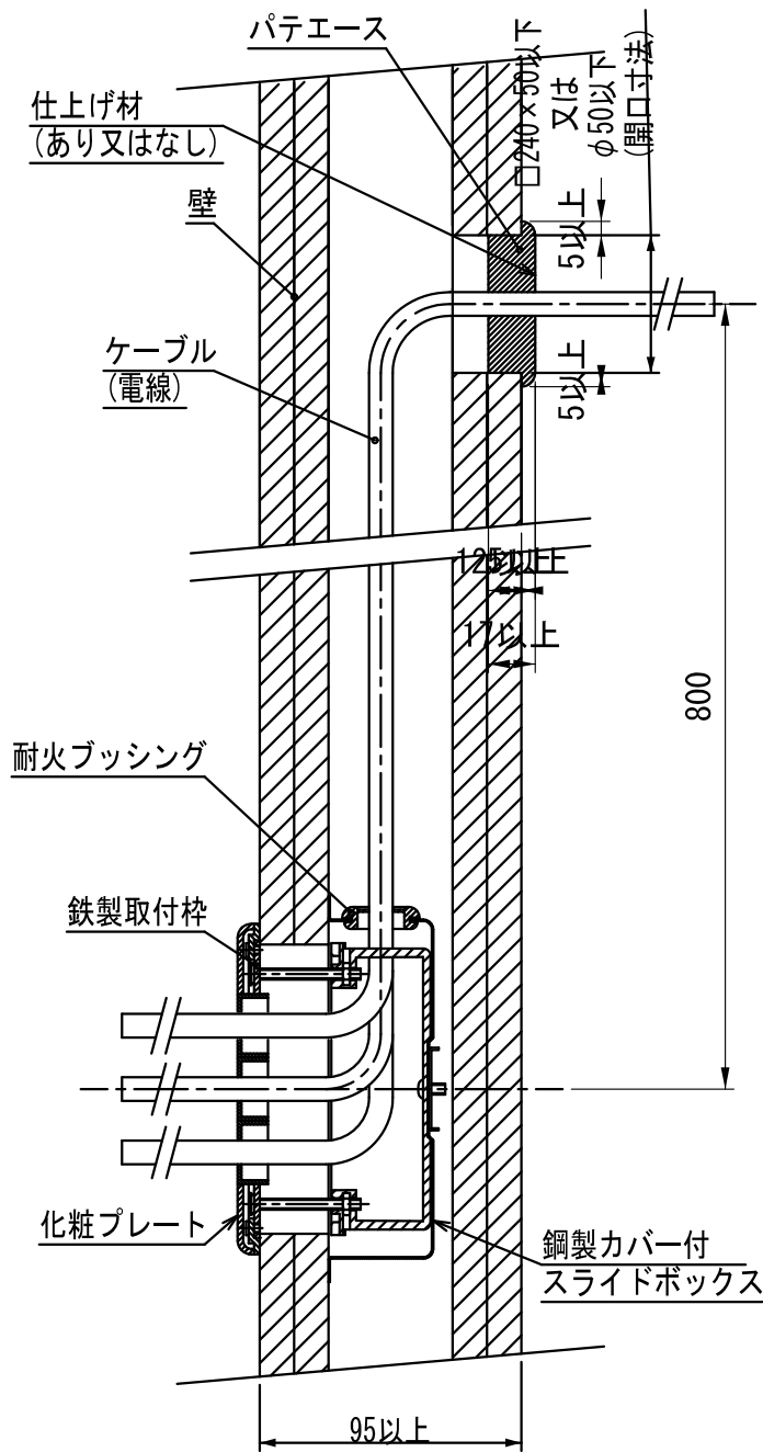
断面図(1/3)
