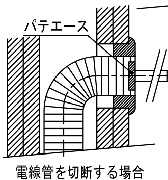
断面図(1/3)
