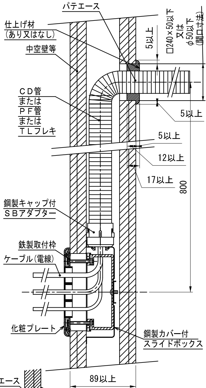
断面図(1/3)
